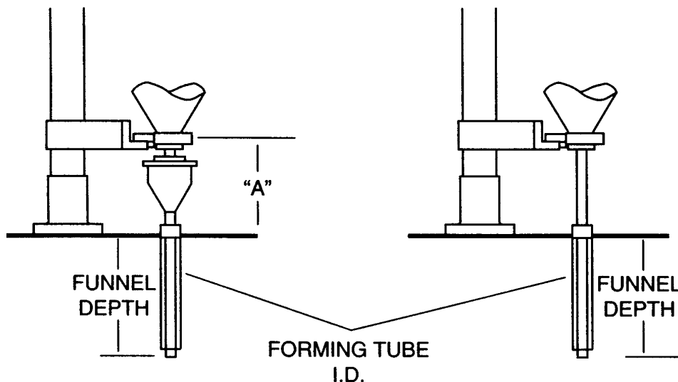
FREE FLOW ASSEMBLY (Granular Products)
